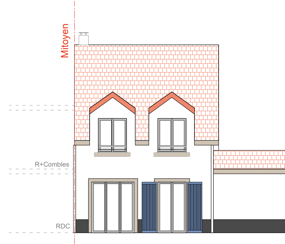
Façade ARRIERE
