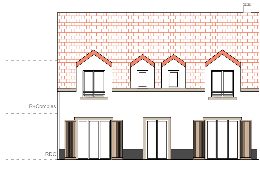
Façade ARRIERE
